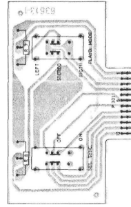
SWITCH BOARD, SOLDER SIDE
