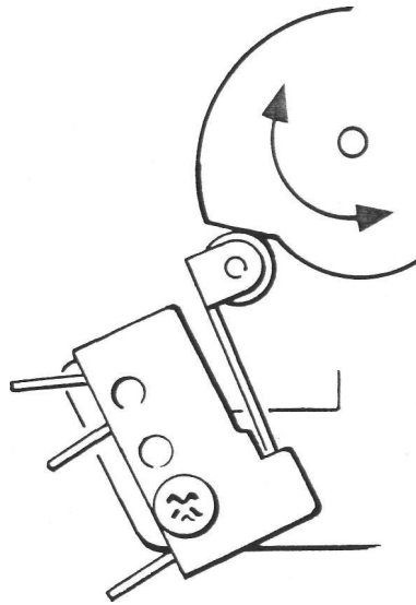
Adjusting the microswitch
