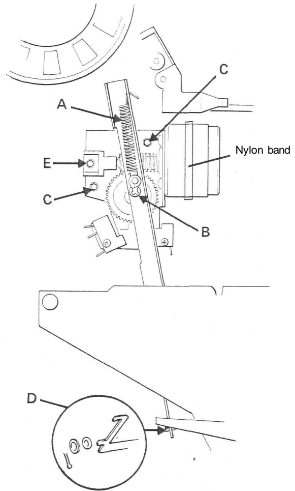
Dismantling the worm-gear motor
