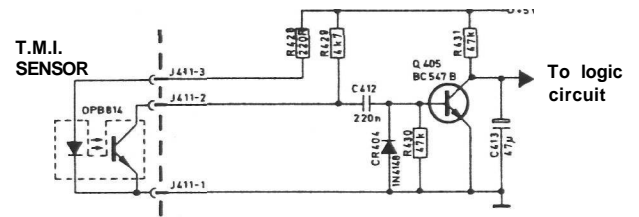
TMI sensor (tape motion indicator) which is a part of the Logic circuit
