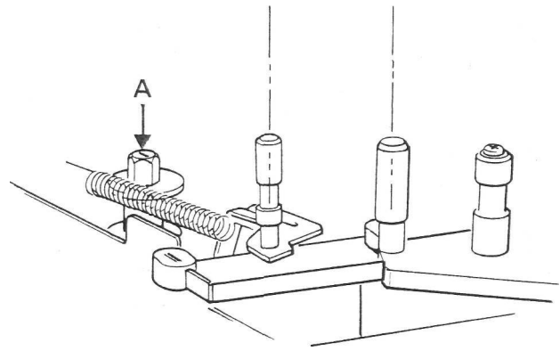
Height adjusting of left tape tension arm
