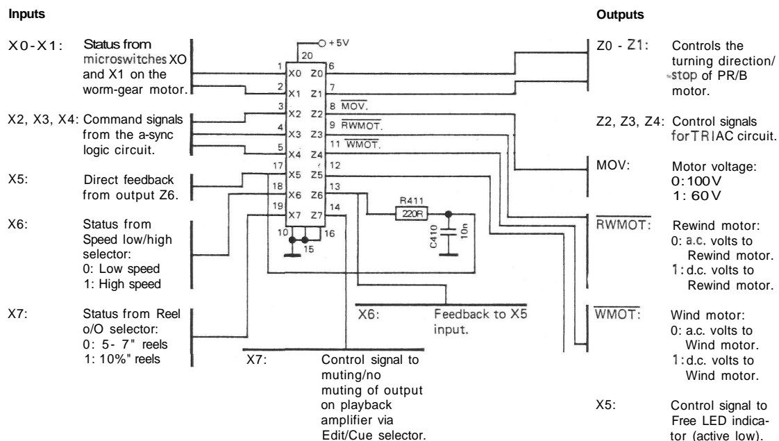
Inputs and Outputs on U3
