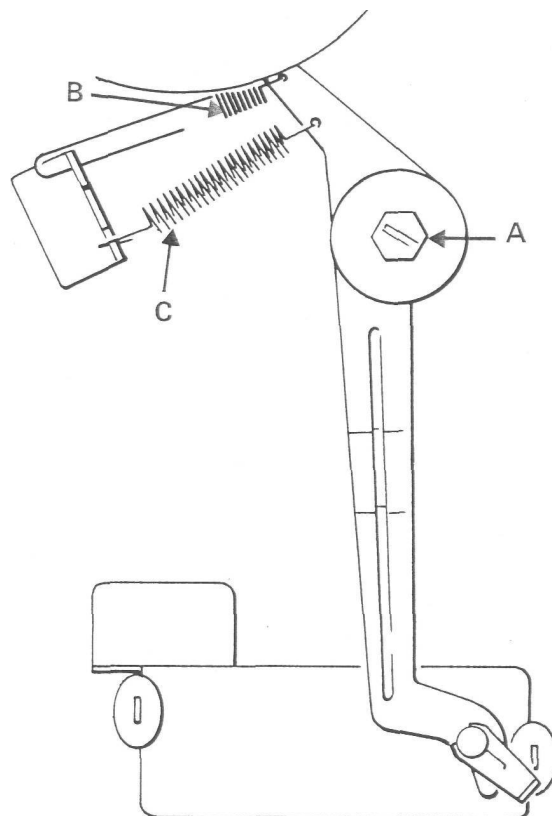
Right tape tension arm
