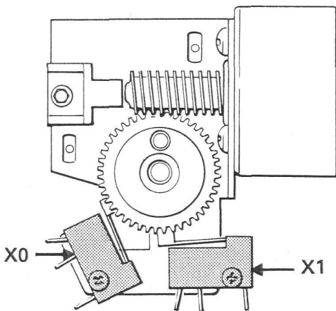
Placing of the microswitches X0 and X1
