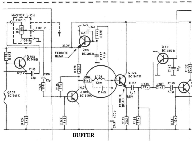
38 kHz trap in the record amplifier
