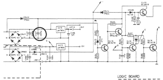
Power On/Off circuit which is a part of the Logic circuit
