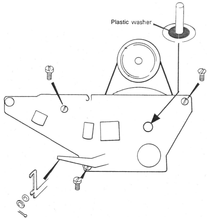
The tape path plate
