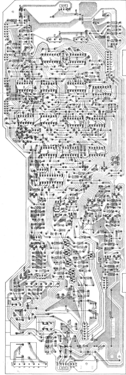
LOGIC BOARD, SOLDER SIDE
