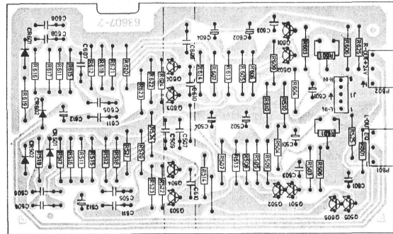
Playback amplifier board (solder side)
