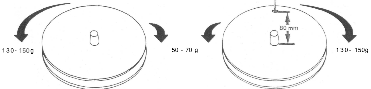
Checking the braking force
