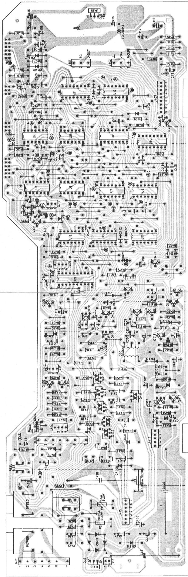
LOGIC BOARD, SOLDER SIDE
