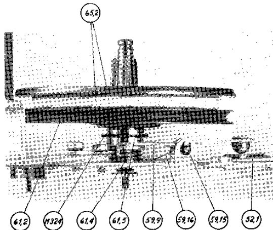
Fig. 12. Supply Turntable, Fast Forward and Normal Forward Drive Positions
