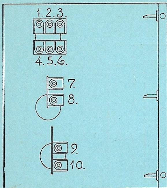
Chassis (underside).
