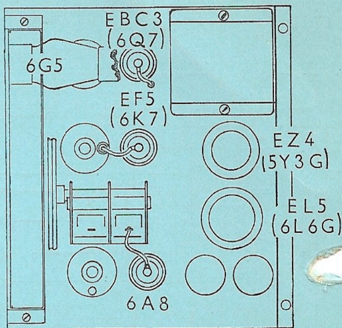
Chassis (overside)
