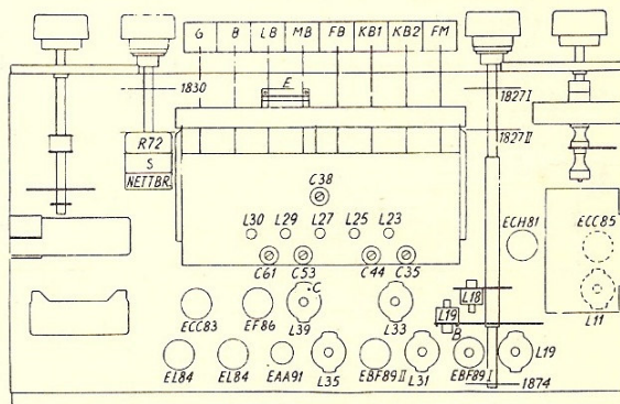
Fig. 2 — Underside
