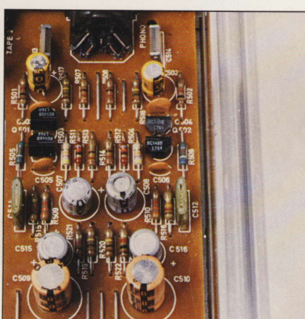
Phono signals are connected directly to a separate RIAA equalizer circuit.
