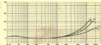
RECORDING CURVES
