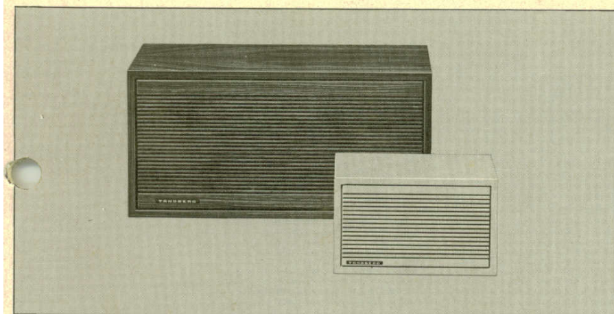
SEPARATE LOUDSPEAKER 9. A high quality remote loudspeaker for kitchen, sitting-room or sleeping-room. Dimensions: Length 16½", height 8½", depth 6". Volume: 8,5 litres. Teak cabinet.
