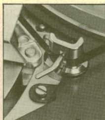
To ease threading of tape the automatic end stop is released when lever is set in position "Free" or "Neutral".
