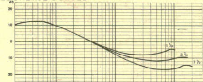
PLAYBACK CURVES
