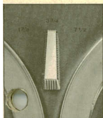
Speed selector for 7\frac{1}{2} " and 3\frac{3}{4} " and 1\frac{7}{8} " ips. can be operated while the recorder is running.
